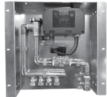
(FLUSH MOUNT)
