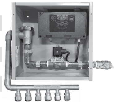
(SURFACE MOUNT)
