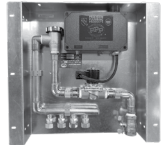
(FLUSH MOUNT)
