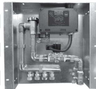
(FLUSH MOUNT)
