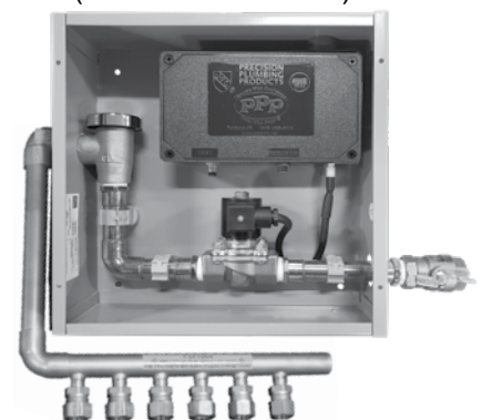
(SURFACE MOUNT)
