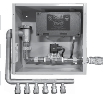
(SURFACE MOUNT)
